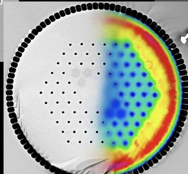
Fiber characterization
